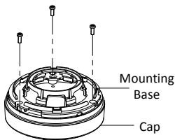
Figure 2-34 Fix Mounting Base
