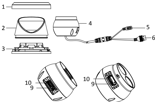
Figure 1-3 Type IV Turret Camera
