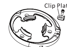
Figure 2-2 Screw the Clip Plate
