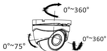
Figure 2-4 3-axis Adjustment
