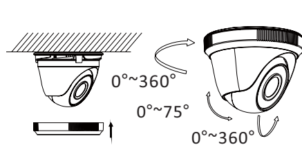
Figure 2-7 3-axis Adjustment
