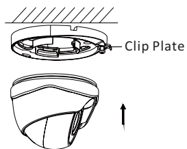
Figure 2-3 Fix the the Camera
