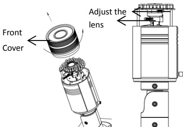
Figure 2-5 Adjust the Lens
