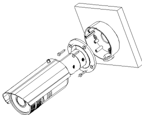
Figure 2-2 Fix the Camera
