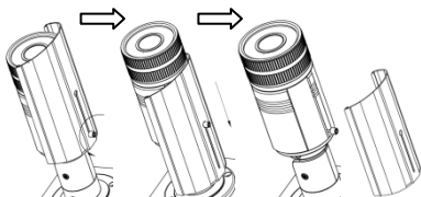
Figure 2-4 Remove the Sun Shield
