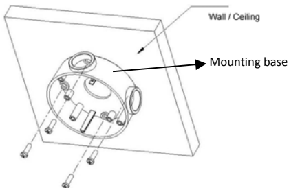
Figure 2-1 Fix the Mounting Base
