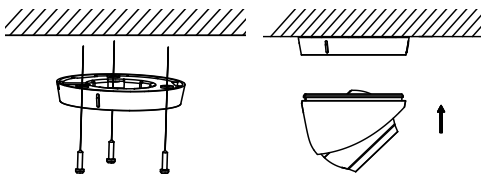
Figure 2-3 Fix the Mounting Base and Camera
